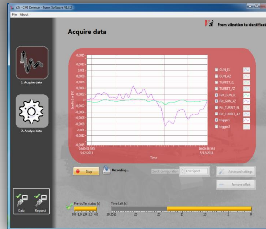
User interface
